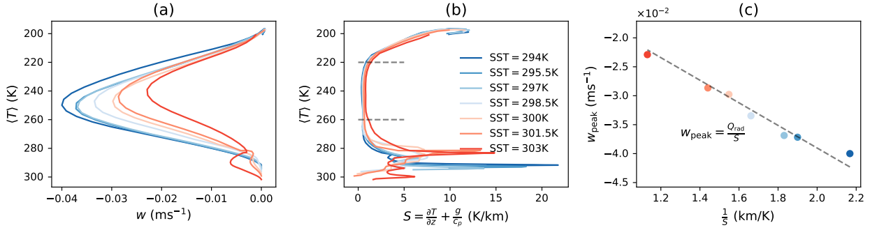
FIG. A1. Tropospheric vertical profiles of (a) vertical velocity w and (b) stability S = \frac{\partial T}{\partial z} + \frac{g}{c_p} in the subsiding branch (i.e. average along x direction above the 10% coldest SSTs) of SAM simulations with the same radiative cooling rate Q_{\text{rad}} = -1.7 K/day but different mean SSTs. Notice here we use temperature as the vertical coordinate. (c) The peak subsiding velocity w_{\text{peak}} as a function of \frac{1}{S} , where S is averaged between the two dotted lines in (b) – the \langle T \rangle = 260 K level and the \langle T \rangle = 220 K level. The dotted line in (c) shows their predicted relation w_{\text{peak}} = \frac{Q_{\text{rad}}}{S} based on theory (details in text).
