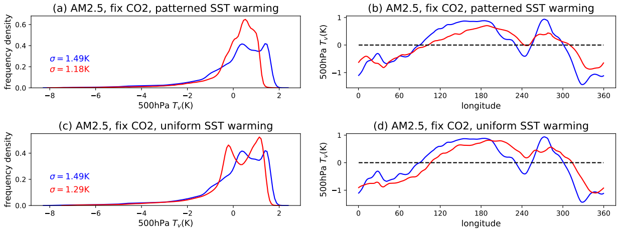
FIG. 2. Robust temperature gradient weakening across scenarios. (a) and (b) Same as Figure 1 (c) and (d) but for AM2.5 forced by the patterned SST warming from the CM2.5-FLOR idealized CO 2 increase simulation and with fixed CO 2 concentration. (c) and (d) Same as Figure 1 (c) and (d) but for AM2.5 forced by uniform SST warming resulting the same global mean SST increase as the CM2.5-FLOR idealized CO 2 increase simulation and with fixed CO 2 concentration. See methods section for simulation details.
