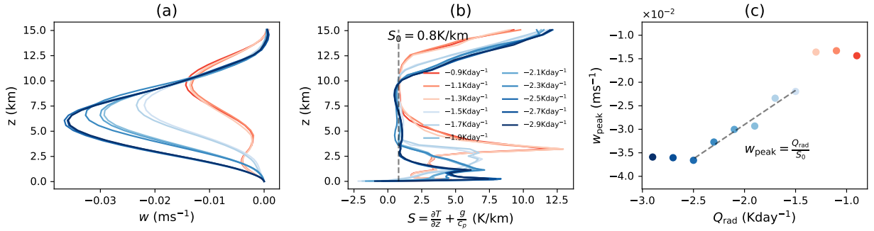
FIG. A2. Tropospheric vertical profiles of (a) vertical velocity w and (b) stability S = \frac{\partial T}{\partial z} + \frac{g}{c_p} in the subsiding branch (i.e. average along x direction above the 20% coldest SSTs) of SAM simulations with the same mean SST of 300 K but different radiative cooling rates Q_{\text{rad}} . (c) The peak subsiding velocity w_{\text{peak}} as a function of the radiative cooling rate Q_{\text{rad}} . The dotted line shows their predicted relation w_{\text{peak}} = \frac{Q_{\text{rad}}}{S_0} based on theory (details in text), where S_0 \approx 0.8 K/km is the constant stability in mid-troposphere for different radiative cooling rates as marked in (b).
