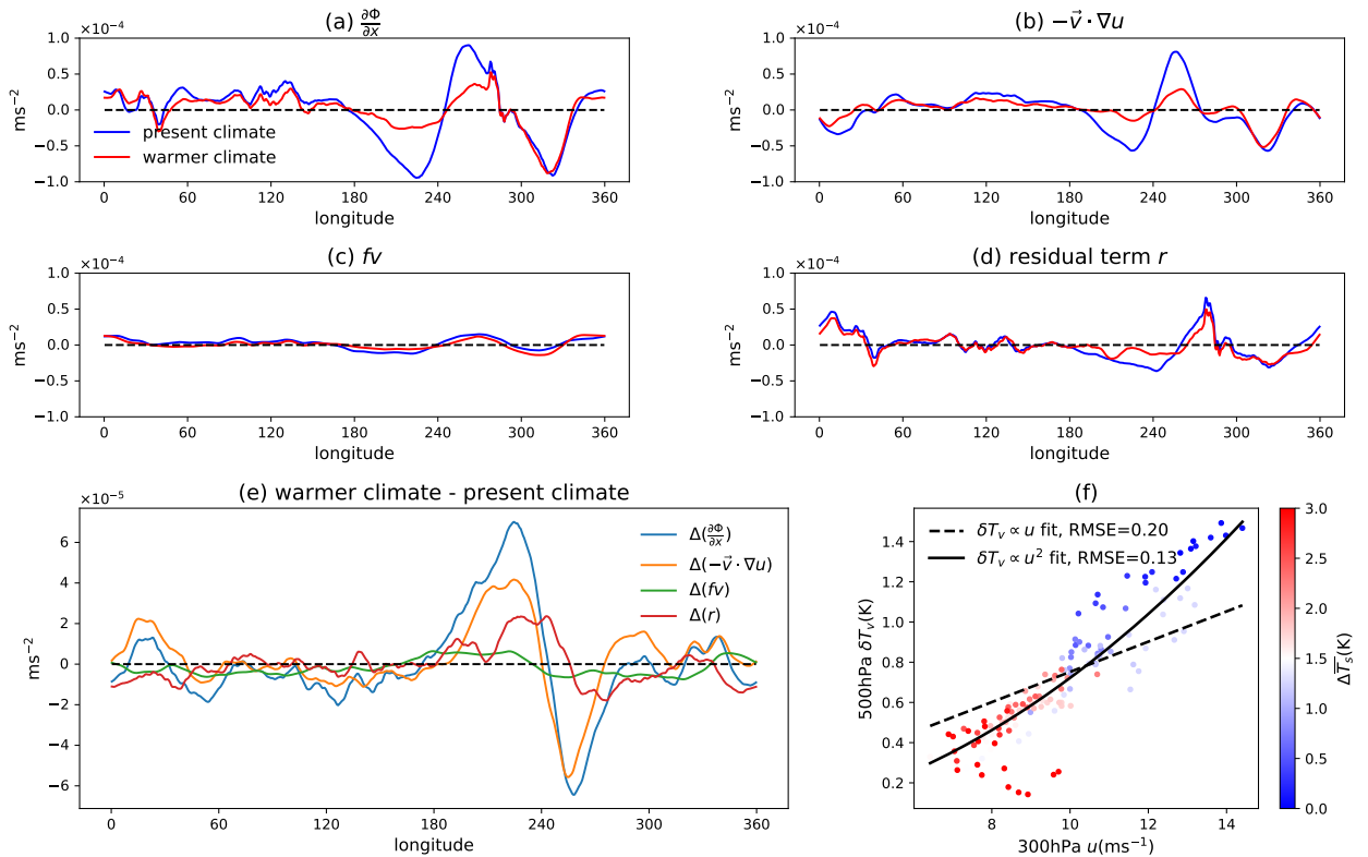
FIG. 3. (a) to (e) 300 hPa zonal momentum budgets close to equator (meridional average between 6^\circ\text{N} to 6^\circ\text{S} ) for present (year 1-10) and warmer (year 131-140) climate in the CM2.5-FLOR idealized \text{CO}_2 increase simulation. (a) (minus) Pressure gradient force \frac{\partial \Phi}{\partial x} . (b) Zonal momentum advection -\vec{v} \cdot \nabla u . (c) Coriolis force fv . (d) The residual term r . (e) Responses (warmer climate minus present climate) of four terms to global warming. All terms are January averages in 10 years. (f) The relation between the 500 hPa virtual temperature difference between the equatorial central Pacific (meridional average between 6^\circ\text{N} to 6^\circ\text{S} at 180^\circ\text{E} ) and the equatorial eastern Pacific (meridional average between 6^\circ\text{N} to 6^\circ\text{S} at 120^\circ\text{W} ), \delta T_v , and the mean zonal wind in this region in the 140-year CM2.5-FLOR idealized \text{CO}_2 increase simulation. Each point is a moving average for ten consecutive Januaries, with the color representing the increase of global mean surface temperature. The dashed/solid curves are linear/quadratic fits (both crossing the origin), and their root mean square errors (RMSEs) are listed.
