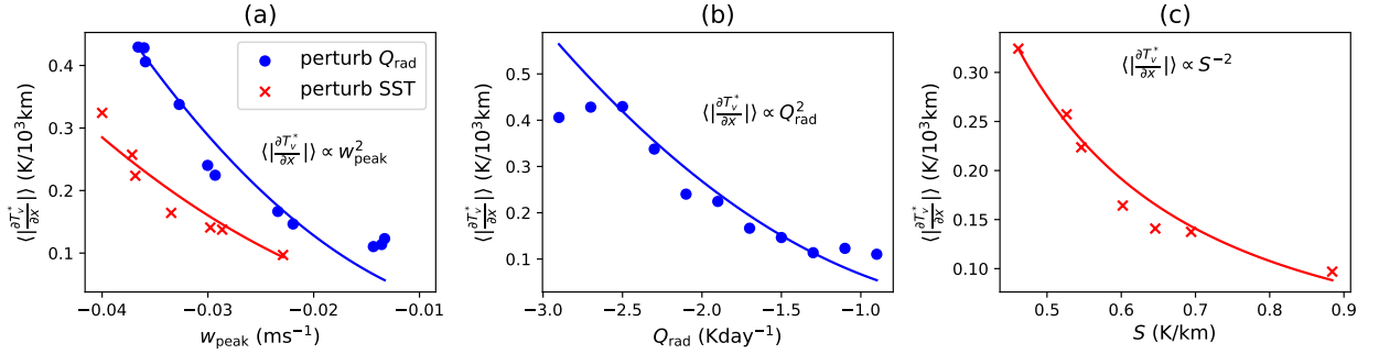
FIG. 5. Weaker circulation causes weaker temperature gradients in CRM simulations. (a) The average (absolute) horizontal T_v^* (defined in equation 7) gradient along x direction, \langle |\frac{\partial T_v^*}{\partial x}| \rangle , as a function of the peak subsiding velocity w_{\text{peak}} in the subsiding branch (details in appendix A) when we change Q_{\text{rad}} under fixed SST (blue) and change SST under fixed Q_{\text{rad}} (red). The dots are model results, and the curves are parabolas going through the origin (equation B8 in appendix B). (b) Same as (a) but showing \langle |\frac{\partial T_v^*}{\partial x}| \rangle as a function of Q_{\text{rad}} when we change Q_{\text{rad}} under fixed SST. (c) Same as (a) but showing \langle |\frac{\partial T_v^*}{\partial x}| \rangle as a function of stability S when we change SST under fixed Q_{\text{rad}} .
