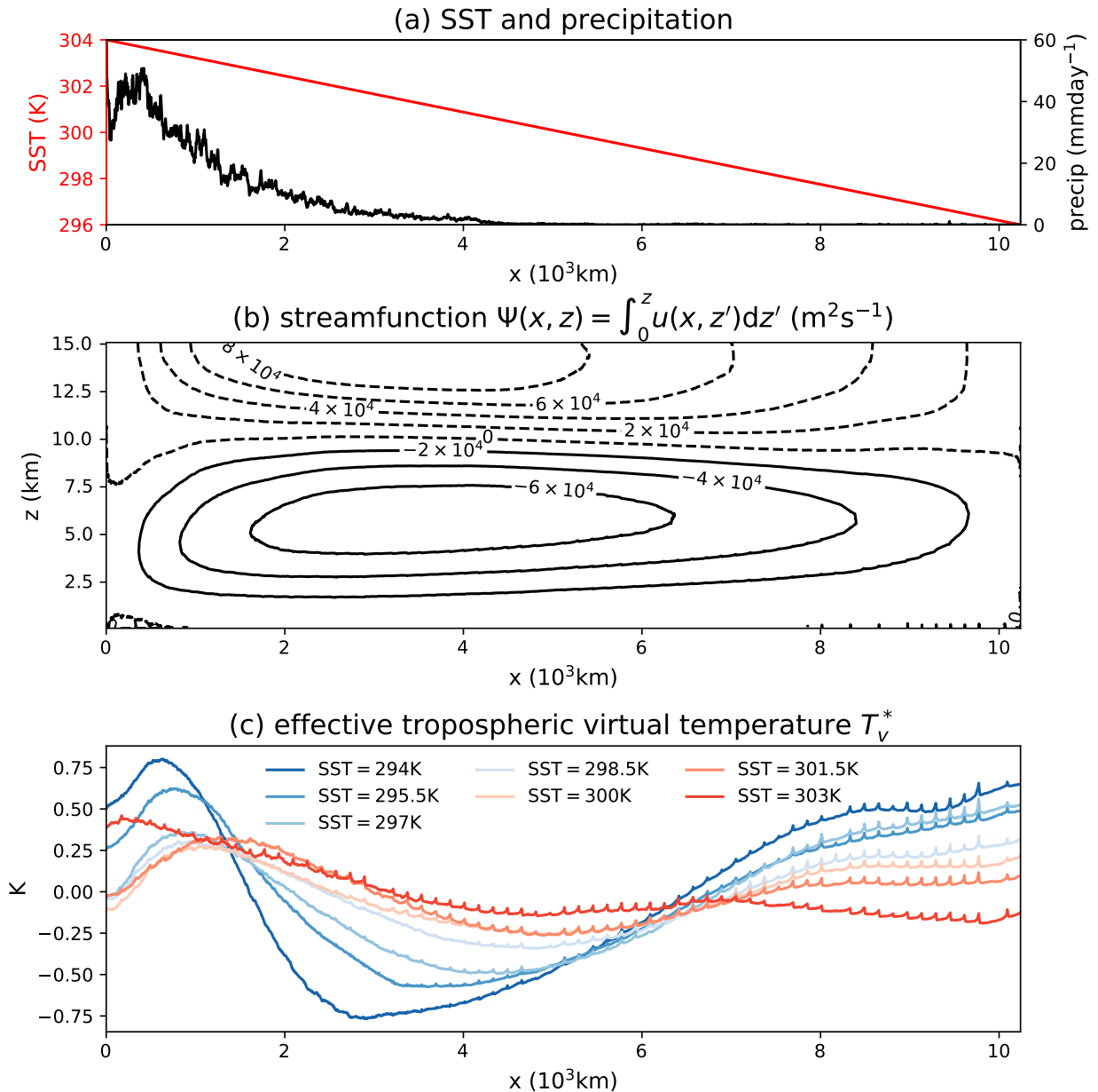
FIG. 4. (a) SST and precipitation profiles and (b) the overturning streamfunction for the simulation with Q_{\text{rad}} = -2.1 K/day and mean SST of 300 K. (c) The effective tropospheric virtual temperature T_v^* (details in text) anomalies (from averages along x direction) in SAM simulations with fixed radiative cooling rate Q_{\text{rad}} = -1.7 K/day but different mean SSTs.
