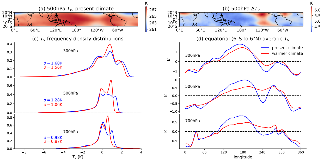
FIG. 1. Weaker temperature gradients in a warmer climate. (a) January climatological mean 500 hPa virtual temperature ( T_v ) in present climate (year 1-10 of the CM2.5-FLOR idealized \text{CO}_2 increase simulation). (b) Response of January climatological mean 500 hPa virtual temperature ( \Delta T_v ) under global warming, calculated as the difference between warmer climate (year 131-140) and present climate (year 1-10). (c) The frequency distributions of T_v anomalies from tropical ( 20^\circ\text{N} - 20^\circ\text{S} ) mean in present climate and warmer climate at 300 hPa, 500 hPa and 700 hPa levels, with their standard deviations \sigma listed. (d) The zonal profiles of T_v anomalies close to equator (meridional average between 6^\circ\text{N} to 6^\circ\text{S} ) in present climate and warmer climate at 300 hPa, 500 hPa and 700 hPa levels.
